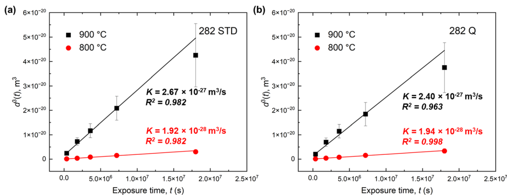
Fig. 13 Plots of average precipitate size, \bar{d}^3(t) , versus exposure time t for alloy STD (a) and alloy Q (b) for temperatures of 800 °C and 900 °C. The coarsening rate constants are determined from the best linear fit of the experimental data.
