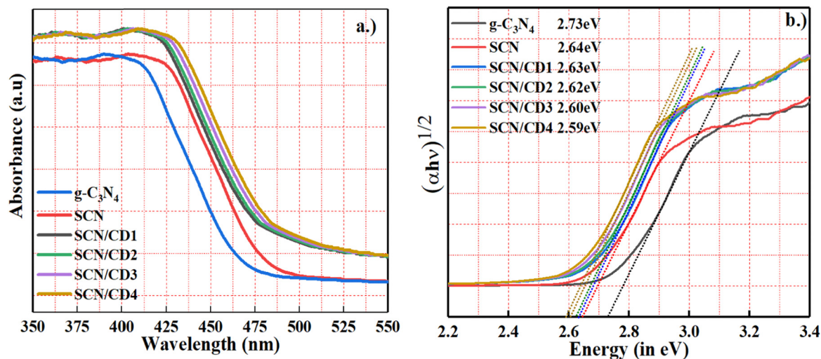
Fig. 5 (a) UV-vis diffuse reflectance of g\text{-C}_3\text{N}_4 , SCN, SCN/CD1, SCN/CD2, SCN/CD3 and SCN/CD4 (b) Tauc plot representing the bandgap energies of g\text{-C}_3\text{N}_4 , SCN, SCN/CD1, SCN/CD2, SCN/CD3 and SCN/CD4.
