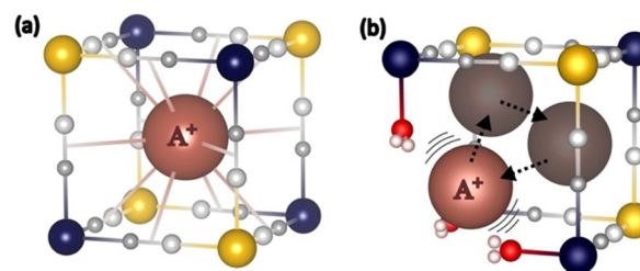
Fig. 3 Scheme of (a) the closed and (b) the open \text{Co}(\text{Co}(\text{OH}_2)_3)_3\text{Fe}_3 Cavities and the proposed positioning for the bigger alkali cations ( \text{Rb}^+ , \text{Cs}^+ ) in each of them.
