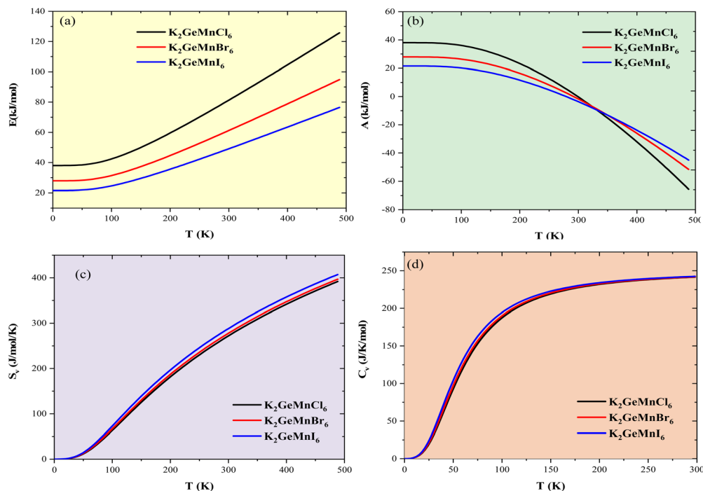
Fig. 5 Thermodynamic vibrational functions for \text{K}_2\text{GeMnX}_6 halide perovskites: (a) vibrational internal energy ( E ), (b) vibrational Helmholtz free energy ( A ), (c) vibrational entropy ( S_v ) and (d) specific heat ( C_v ) against a selected range of temperature.
