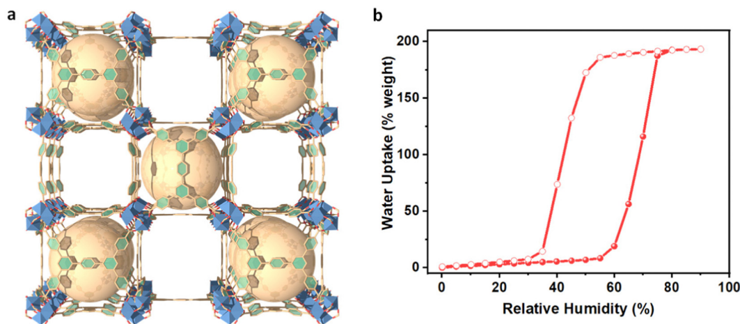
Fig. 1 (a) Crystal structure of Super-adsorbent Cr- soe -MOF-1. (b) Water sorption isotherm at 298 K for activated Cr- soe -MOF-1.
