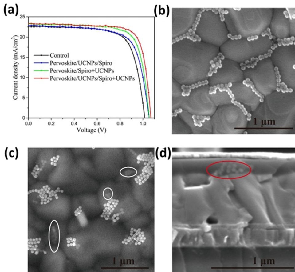
Fig. 15 (a) J - V characteristics of several types of PSCs. Top-view SEM images of (b) perovskite/UCNP film and (c) perovskite/UCNP/spiro + UCNP film. (d) Cross-sectional SEM images of the PSC with the structure of ITO/SnO 2 /perovskite/UCNPs/spiro + UCNPs/Au. Reprinted with permission from the American Chemical Society. 93
