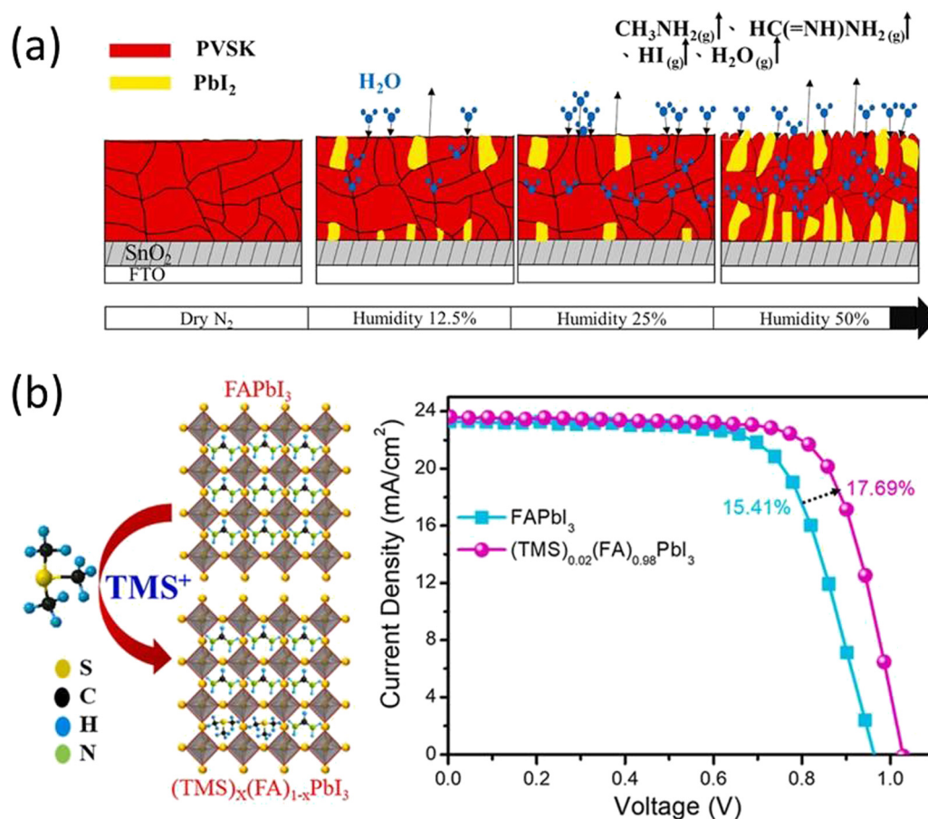
Fig. 2 (a) Water molecules in contact with (Cs 0.05 FA 0.85 MA 0.15 Pb(I 0.85 Br 0.15 ) 3 ) perovskite crystal grain boundaries form a hydrated phase; PVSK in the figure. Continuous heating during the annealing process returns partially hydrated phases to the original perovskite phase, while a portion of the samples underwent degradation during the annealing process, returning partially hydrated phases to the original perovskite phase, while a portion of the samples underwent degradation, resulting in the formation of large quantities of CH 3 NH 2 , HC(=NH)NH 2 , HI, PbI 2 , PbBr 2 , and H 2 O. Increasing the humidity levels to 50% accelerated degradation, resulting in the formation of large quantities of CH 3 NH 2 , HC(=NH)NH 2 , and PbI 2 . Reproduced from ref. 69 with permission from John Wiley and Sons, copyright 2022. (b) Schematic crystal structure and JV plots of FAPbI 3 before and after TMS + incorporation. Reproduced from ref. 73 with permission from Elsevier, copyright 2022.
