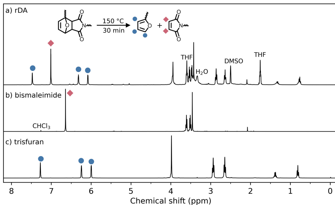
Fig. 5 ^1\text{H-NMR} spectra of (a) the DA-adduct after 30 minutes at 150 °C in \text{DMSO-d}_6 , (b) the bismaleimide monomer recorded in \text{CDCl}_3 and (c) the trisfuran monomer recorded in \text{CDCl}_3 . The THF observed in spectrum (a) is attributed to residual THF after the swelling tests.
