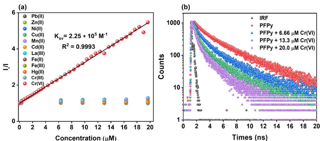
Fig. 3 (a) Determination of the Stern–Volmer constant ( K_{\text{SV}} ) for \text{Cr(VI)} in water, and 2D S–V plots for various metal ions; (b) TRPL spectra of PFPy (6.66 \mu\text{M} ) with different concentrations of \text{Cr(VI)} (6.66, 13.3 and 20.0 \mu\text{M} ) in water, where IRF denotes the “Instrument Response Function”.
