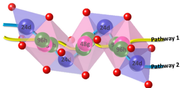
Fig. 4 The lithium diffusion pathway in the cubic LLZO crystal. The diffusion follows two paths. Pathway 1: 96h–48g–96h involving only octahedral sites (yellow line). Pathway 2: 24d–96h–48g–96h–24d involving both octahedral and tetrahedral sites (blue line).
