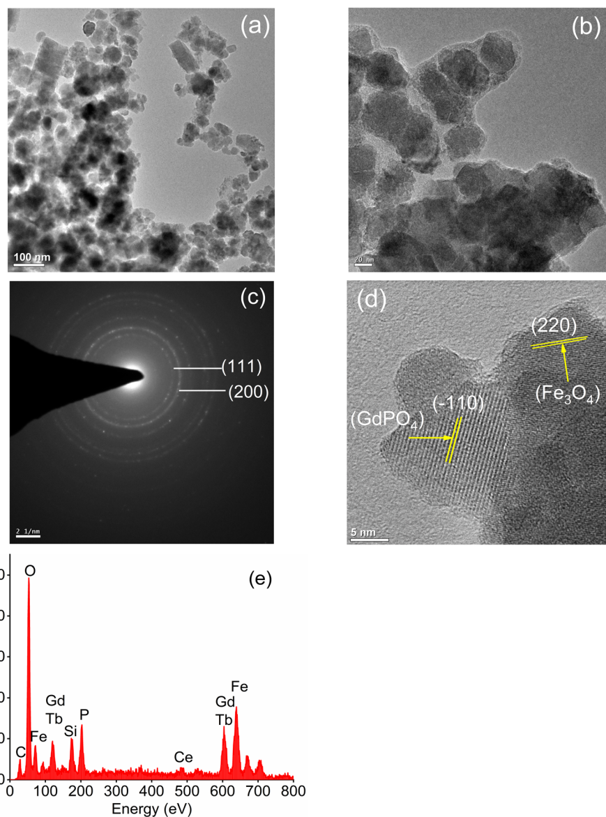
Fig. 2 TEM images of (a) \text{Fe}_3\text{O}_4 nanoparticles and (b) CMC functionalized \text{Fe}_3\text{O}_4@\text{SiO}_2@\text{GdPO}_4:\text{Tb}^{3+},\text{Ce}^{3+} nanocomposites. (c) SAED pattern of \text{Fe}_3\text{O}_4 nanoparticles, (d) HRTEM image and (e) EDS spectra of CMC functionalized \text{Fe}_3\text{O}_4@\text{SiO}_2@\text{GdPO}_4:\text{Tb}^{3+},\text{Ce}^{3+} nanocomposites.
