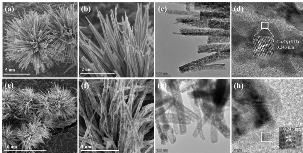
Fig. 2 SEM images of (a and b) \text{Co}_3\text{O}_4 and (e and f) \text{CoP} . TEM images of (c) \text{Co}_3\text{O}_4 and (g) \text{CoP} . HRTEM images of (d) \text{Co}_3\text{O}_4 and (h) \text{CoP} .
