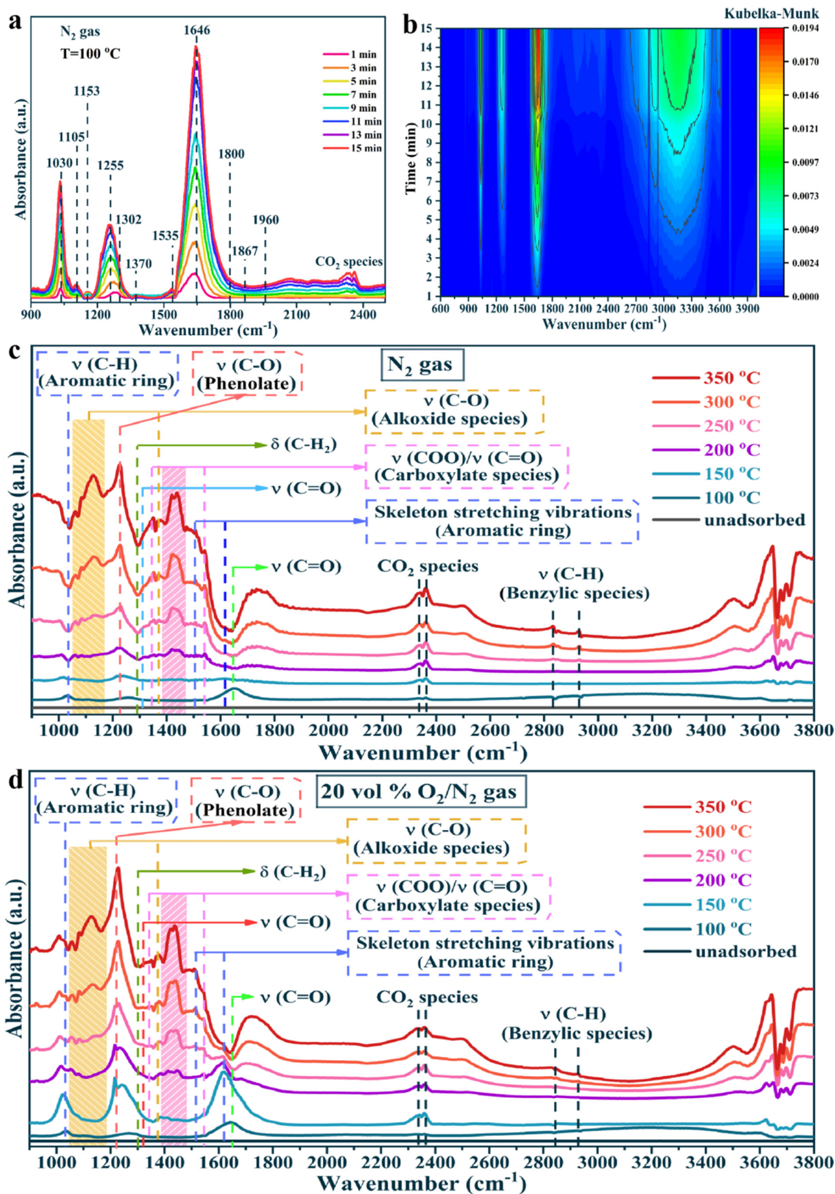
Fig. 9 In situ DRIFTS spectra of toluene adsorption (a and b) for Pt t NC@CeO 2 catalyst at 100 °C for different times under pure N 2 gas flow and the in situ DRIFTS spectra of Pt t NC@CeO 2 catalyst for different reaction temperatures with toluene/N 2 gas (c) and toluene/air gas (d).
