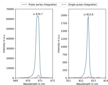
Fig. 2 Influence of the integration setting on the intensity of selected lithium emission lines ( 1 \text{ mg L}^{-1} Li) comparing measurement settings A (pulse series integration) and D (single pulse integration).
