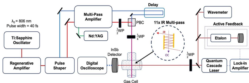
Fig. 1 Schematic diagram of the optical centrifuge and high-resolution transient IR absorption spectrometer. The pair of optical centrifuge pulses have orthogonal linear polarization after the \frac{1}{2} -wave plate ( \frac{1}{2} WP) and opposite circular polarization after the \frac{1}{4} -wave plate ( \frac{1}{4} WP). The IR \frac{1}{2} -wave plate is used to control the polarization of the IR probe.
