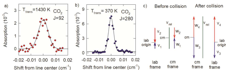
Fig. 11 Doppler-broadened line profiles for \text{CO}_2 (a) J = 92 and (b) J = 280 at 200 ns following the optical centrifuge pulse. (c) Velocity vectors in the lab frame ( v ) and center of mass (cm) frame ( w ) for a collision with b = 0 of an optically centrifuged molecule and a thermal bath molecule, before (1, 2) and after (3, 4) collisional energy transfer.
