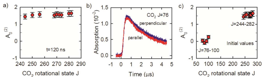
Fig. 8 (a) Alignment moment A_0^{(2)} of optically centrifuged \text{CO}_2 J = 244 – 282 at t = 120 ns. (b) Polarization-sensitive transient IR absorption signals for J = 76 . (c) Comparison of initial A_0^{(2)} values for \text{CO}_2 J = 244 – 282 and J = 76 – 100 .
