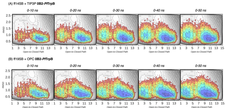
Fig. 4 Estimated FEL of OB2-PfTrpB . The estimated FEL from the accumulated multiple replica nanosecond timescale MD simulations performed starting at the ensemble of template-based AF2 predictions, is shown in colour on top of the previously reconstructed FEL of the PfTrpB variant (shown in grey scale). 19 FELs are displayed every 10 ns of MD simulation time and using two different combinations of forcefield and water model: (A) ff14SB and TIP3P water, and (B) ff19SB and OPC water. The x axis denotes the ensemble of structures generated from X-ray data for the open-to-closed transition of the COMM domain, which ranges from 1–5 (open, O), 6–10 (partially closed, PC), to 11–15 (closed, C), the y axis is the mean square deviation (MSD, in Å 2 ) from the path of O-to-C structures generated. Most stable conformations are shown in blue, whereas higher energy regions are shown in red.
