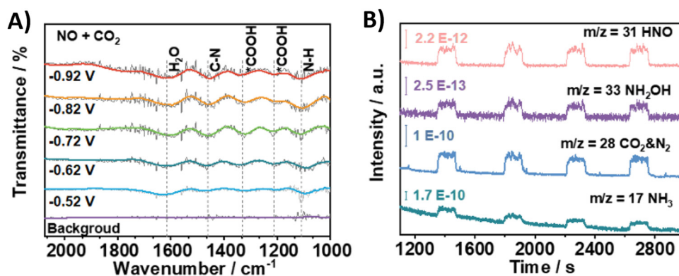
Fig. 19 Mechanistic investigations involving the formation of \text{*H}_2\text{NCO} using the Zn NBs catalyst. (A) In situ ATR-FTIR spectra at different potentials with NO + CO 2 as the feed gas. (B) Online DEMS measurements. Adapted from ref. 200.
