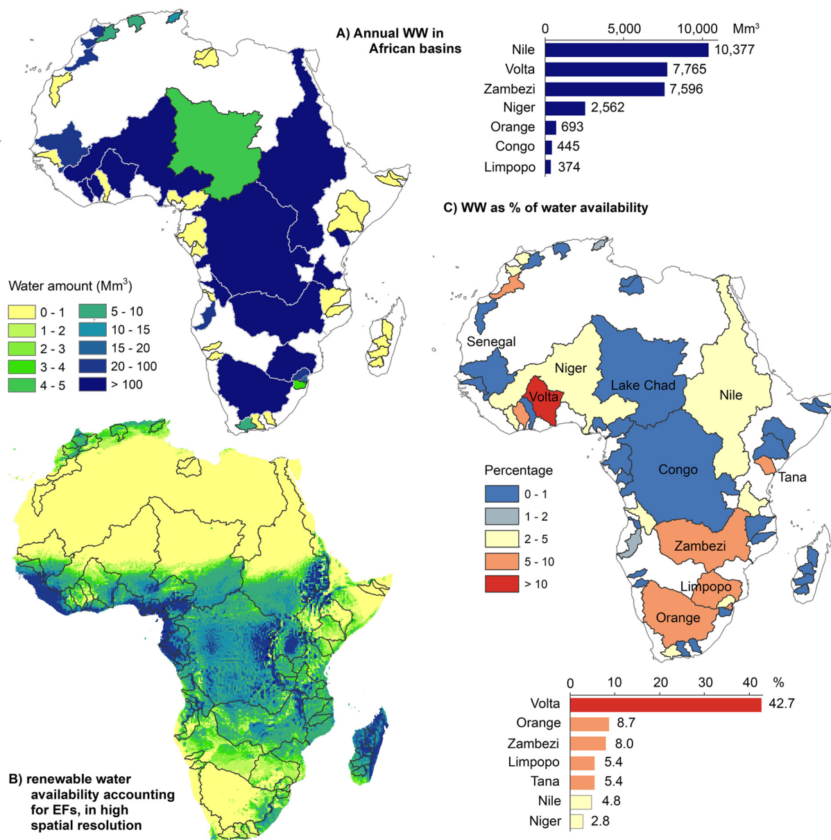
Fig. 4 Annual water withdrawal in major African river basins. A) Annual WW in \text{Mm}^3 highlighting the seven basins with the highest amounts; B) annual renewable water availability (natural water availability minus EFs) in high spatial resolution (0.1 degrees) (source Vanham et al. 21 ); C) WW as percentage to renewable water availability per basin, highlighting selected basins with the highest amounts. Detailed results for all basins in SI_Results.
