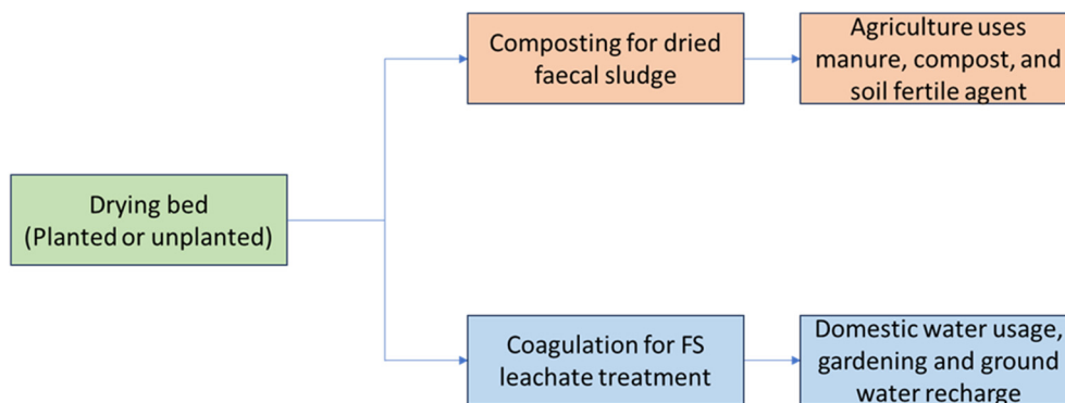
Fig. 15 Suggested line of treatment for FS in this case study.
