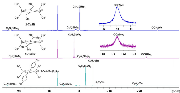
Fig. 3 ^1\text{H} NMR 298 K spectra in \text{C}_6\text{D}_6 of 2-Ce/Et, 2-Ce/ i^t\text{Pr} , and 2-Ce/ \text{C}_6\text{H}_4\text{-}^t\text{Bu} including insets of significantly upfield methylene and methine ^1\text{H} signals of 2-Ce/Et and 2-Ce/ i^t\text{Pr} , respectively.
