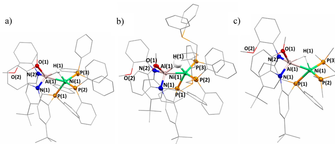
Fig. 2 Solid-state structures of (a) 2\text{-(PPh}_3)_2 , (b) 2\text{-(dppe)}_2 , and (c) 2\text{-(PMe}_3)_2 . Hydrogen atoms on ligands are excluded for clarity. Mixed wire-frame/ellipsoid view used for clarity.
