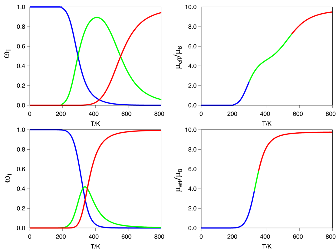
Fig. 3 (Left) Spin state populations ( \omega_i ) for the ([\text{Fe}_2(\text{L}_1)_3]@X)^{3+} systems ( X = \text{F}^- with \rho = -0.31 , top, X = \text{Br}^- , \rho = -0.06 , bottom): i = [\text{LS-LS}] (blue), [\text{HS-LS}] (green) and [\text{HS-HS}] (red) populations. (Right) Estimation of the magnetic moment computed from the corresponding spin-state populations.
