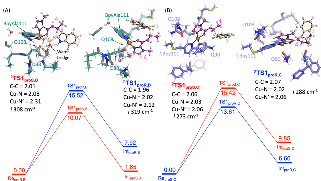
Fig. 5 Potential energy landscape for the Friedel–Crafts alkylation by A) SCP_Q11BpyAla and B) SCP_Q111CBpy. Energy values are in kcal mol -1 . The optimized geometric structures of the transitions are shown on the left and right of free energy landscape with their important bond lengths in Å. The imaginary frequency represents the stretching vibration of C–C bonds between 3 and 4 for each transition state.
