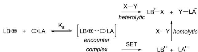
Scheme 1 The equilibrium between a Lewis base (LB) and Lewis acid (LA) and the encounter complex with equilibrium constant K_a . Subsequently, the synergistic, closed-shell activation of substrate X–Y can occur or potentially single electron transfer (SET) to afford a radical pair that can homolytically cleave X–Y.
