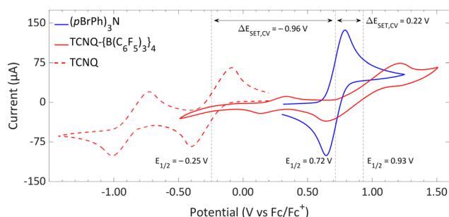
Fig. 11 CVs of \text{TCNQ}\cdot\{\text{B}(\text{C}_6\text{F}_5)_3\}_4 , TCNQ and (p\text{BrPh})_3\text{N} in DCM, showing reversible redox events. For TCNQ and (p\text{BrPh})_3\text{N} [n\text{Bu}_4\text{N}][\text{PF}_6] (0.1 M) was added as electrolyte, while for \text{TCNQ}\cdot\{\text{B}(\text{C}_6\text{F}_5)_3\}_4 no additional electrolyte was used. For clarity reasons part of the CV of TCNQ and (p\text{BrPh})_3\text{N} has been omitted. The full spectra and experimental details are reported in the ESI.†
