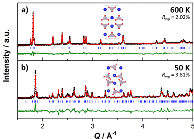
Fig. 2 Rietveld refinements to the neutron Bragg data of TlTcO 4 , collected on the POWGEN diffractometer at (a) 600 K refined to the tetragonal I 41 / amd space group, and (b) 50 K refined to the orthorhombic Pnma space group. The black circles represent the data, the red line represents the fit to the data, the green line represents the difference between the data and the fit, and the blue dashes represent the space group-allowed reflections.
