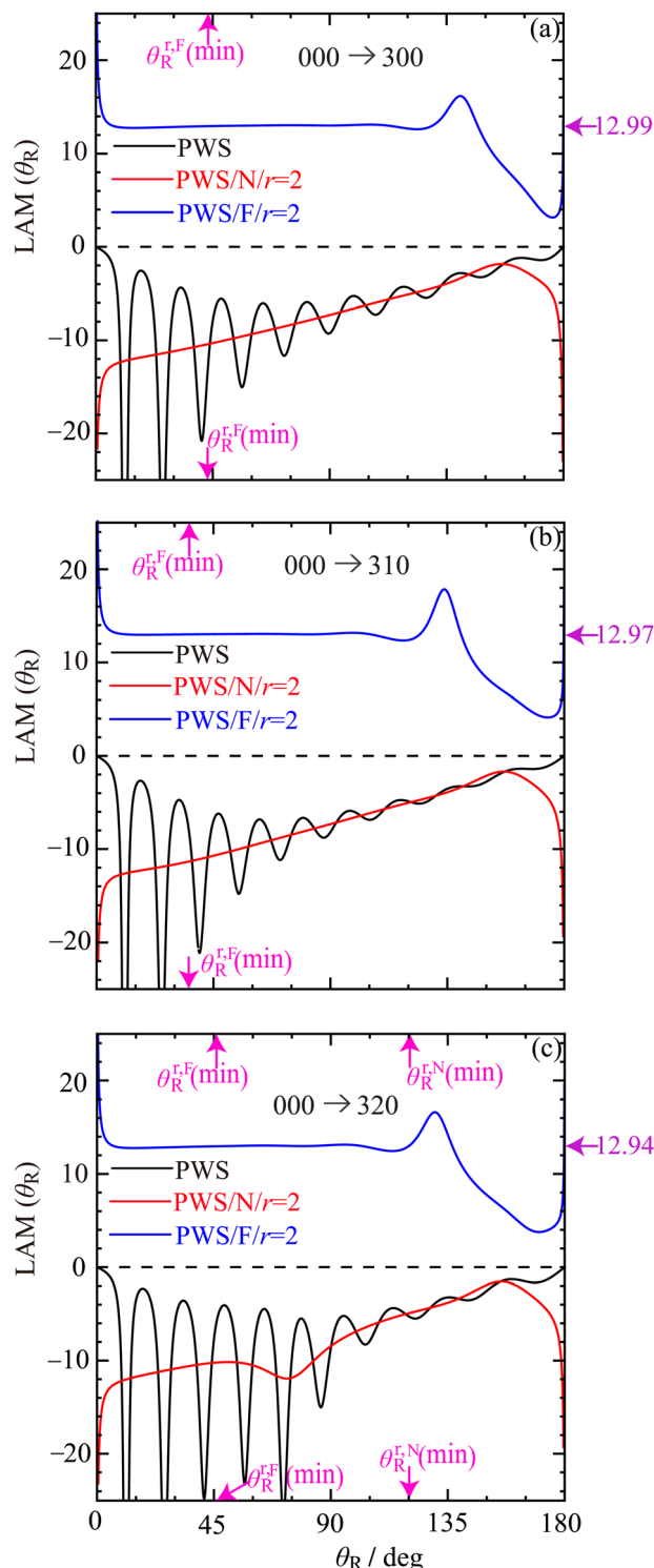
Fig. 5 Plots of full and N, F LAM( \theta_R ) versus \theta_R at E_{\text{trans}} = 62.09 meV. Black curve: PWS. Red curve: PWS/N/ r = 2 . Blue curve: PWS/F/ r = 2 . The purple arrow pointing towards the right ordinate shows, \text{Re } J_0 + 1/2 . The locations of the nearside (N) and farside (F) rainbow angles, \theta_R^{F,\text{N}}(\text{min}) and \theta_R^{F,\text{N}}(\text{min}) respectively, are shown as pink arrows pointing towards the abscissa. For clarity, not all rainbow angles in Fig. 6 are shown. The transitions are: (a) 000 \rightarrow 300 , (b) 000 \rightarrow 310 , (c) 000 \rightarrow 320 .
