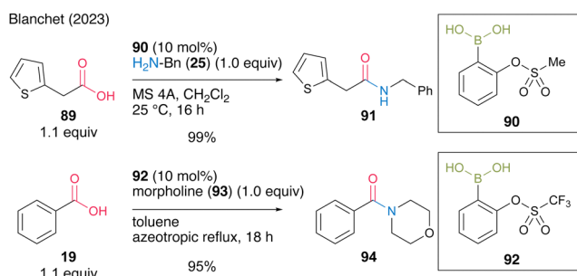
Scheme 14 2-Sulfonatobenzenboronic acid-catalyzed amidation reported by Blanchet. 31
