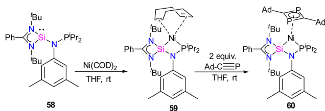
Scheme 21 (a) Synthesis of phosphine functionalized silylene-Ni(0) complex 59 . (b) The reactivity of 59 with \text{Ad-C}\equiv\text{P} .
