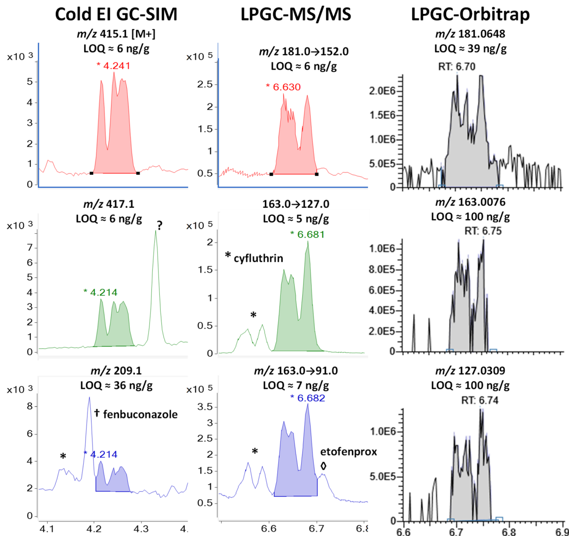
Fig. 7 Comparison in the analysis of 100 ng g -1 (75 pg injected) cypermethrin in the barley extract using different fast GC-MS techniques.
