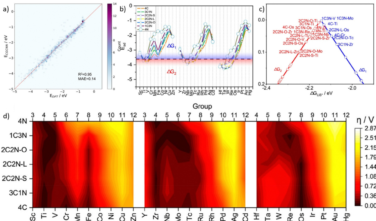
Fig. 10 Taken from Fig. 3 and 4 in Lian et al. 211 (a) DFT calculated and machine learning predicted adsorption energy of Li-polysulfides, (b) predicted adsorption energy of LiS^* , (c) volcano plots for catalysts with an overpotential lower than 0.1 V, and (d) heat map of the predicted overpotential of different SACs. Reproduced with permission. 211 Reprinted (adapted) with permission from ref. 211. Copyright 2021 American Chemical Society.
