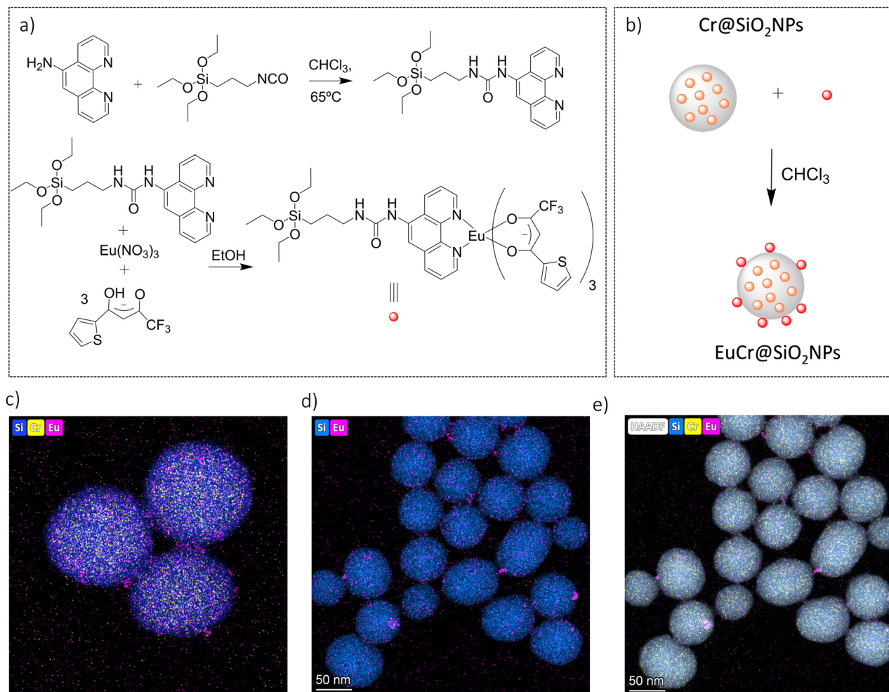
Fig. 6 (a) Synthetic steps for the preparation of the Eu III complex. (b) Schematic synthesis of (\lambda/\lambda\delta) -EuCr@SiO 2 NPs (c) TEM image of the functionalized nanoparticle. (d) and (e) HAADF-STEM compositional mapping image of \lambda\lambda -EuCr@SiO 2 NPs.
