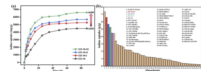
Fig. 1 (a) Iodine adsorption isotherms of ZIF-90 and ZIF-90-I-ZIF-90-III at 75 °C under ambient pressure, and (b) comparison of the iodine vapor adsorption capacity by reported metal-organic frameworks and our materials.
