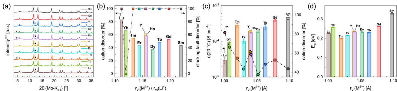
Fig. 5 (a) PXR diffraction patterns and (b) degrees of intra-layer cation disorder and stacking fault disorder obtained from Rietveld refinements of the different \text{Li}_3\text{MI}_6 . Asterisks and diamonds correspond to impurities of \text{MOI} and \text{MI}_3 , respectively. In (c) ionic conductivities at 20 °C with intra-layer cation disorder and in (d) activation energies for ion diffusion obtained from EIS are shown as a function of the ionic radii 43–45 of the rare earth metal cations.
