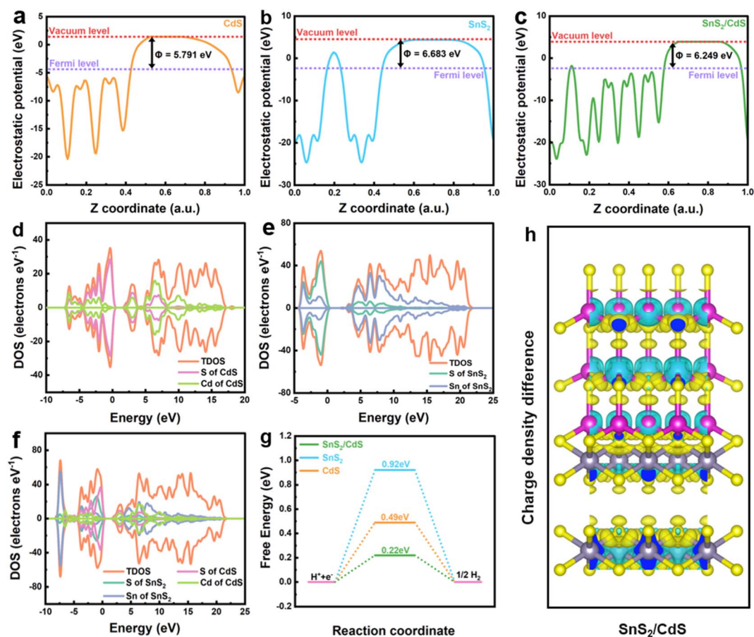
Fig. 9 (a–c) Work function and (d–f) density of state plots, (g) hydrogen adsorption free energy diagram of \text{CdS} (002), \text{SnS}_2 (100), and \text{SnS}_2/\text{CdS} heterostructures interface, and (h) charge density difference diagram for \text{SnS}_2/\text{CdS} heterostructures.
