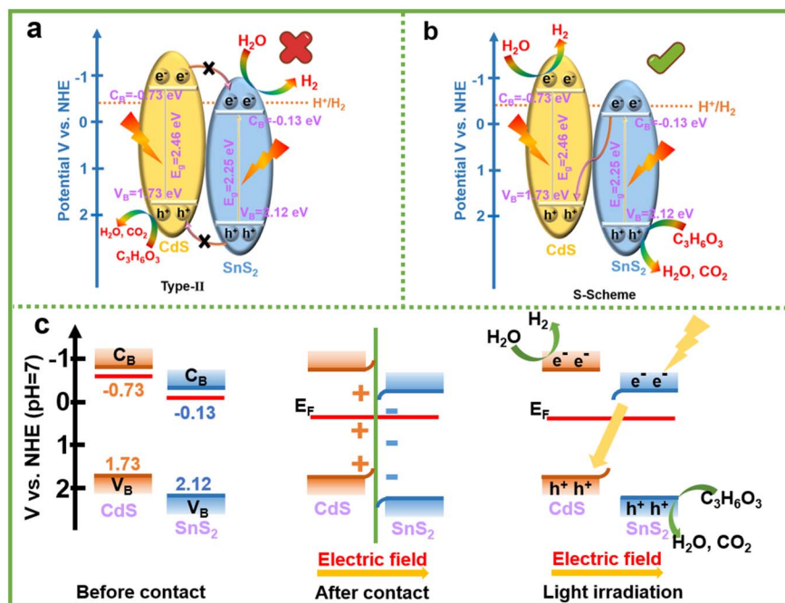
Fig. 8 (a) Type-II and (b and c) S-scheme illustration of the possible charge transfer processes in the \text{SnS}_2/\text{CdS} heterostructures.
