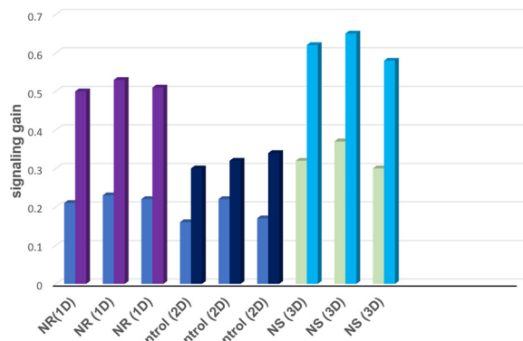
Fig. 7 Shows repeatability results for three freshly prepared E-AB sensors 1D, 2D, and 3D. The left bar represents the initial signal of the E-AB sensor, and the right bar is the signal gain after target hybridization.
