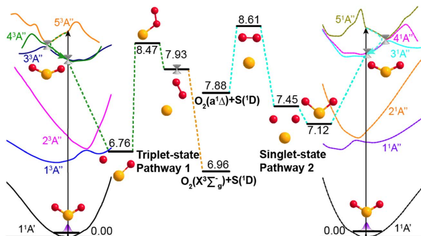
Fig. 4 Dissociation pathways of \text{SO}_2 leading to \text{O}_2(\text{X}^3\Sigma_g^-) + \text{S}^1\text{D} products via the triplet state manifold (left) and to \text{O}_2(\text{a}^1\Delta_g) + \text{S}^1\text{D} products via the singlet state manifold. The schematics of the simplified PECs for the ground and the first five excited states of ^3\text{A}'' symmetry (left) and the first five states of ^1\text{A}'' symmetry (right) support different paths leading to \text{S} + \text{O}_2 product formation. Dashed arrows indicate possible non-adiabatic pathways and the geometries and energies (in eV) of key intermediate structures along the dissociation pathways are also indicated. The horizontal axis represents the reaction coordinate, and the vertical axis is the potential energy (in eV).
