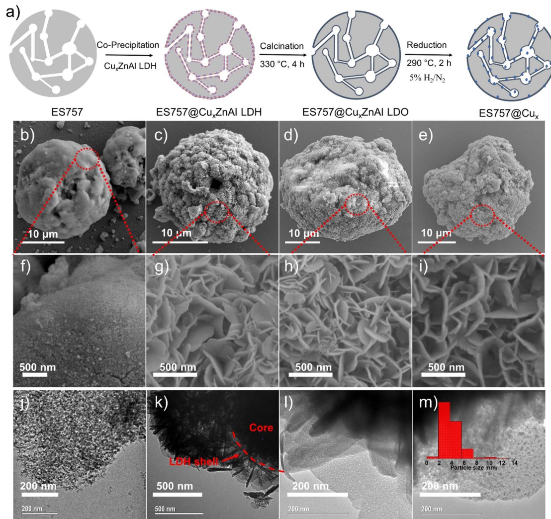
Fig. 1 (a) Synthesis scheme of Cu nanoparticles from ES757@Cu x ZnAl LDH. SEM images of (b and f) ES757; (c and g) ES757@Cu 1.3 ZnAl LDH; (d and h) ES757@Cu 1.3 ZnAl LDO and (e and i) ES757@Cu x . TEM images of (j) ES757; (k) ES757@Cu 1.3 ZnAl LDH; (l) shell of ES757@Cu 1.3 ZnAl LDO; (m) shell of ES757@Cu 1.3 .
