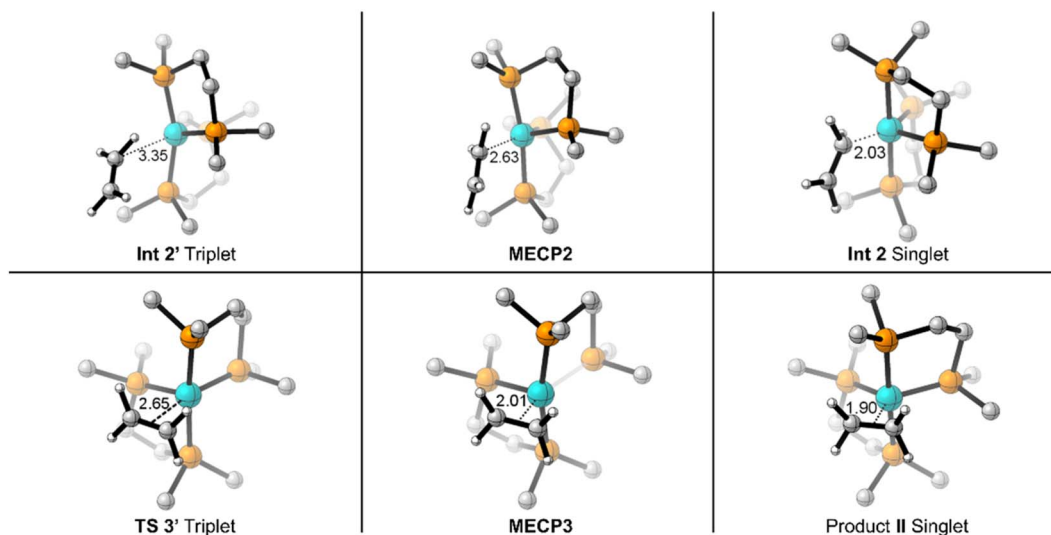
Fig. 3 3D depiction of M06-L optimized geometries for reaction between (\text{DMPE})_2\text{Fe} and ethylene with key bond/coordination distances (in \text{Å} ).
