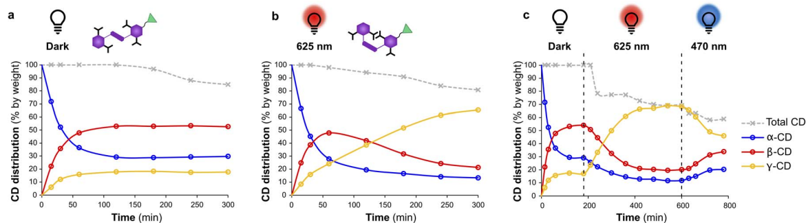
Fig. 5 Distribution of \alpha -, \beta -, and \gamma -CD as function of time for enzymatic reactions starting from \alpha -CD (10 mg mL -1 ) with CGTase (65 \mu\text{L} mL -1 ) in sodium phosphate buffer (100 mM, pH 7.5) in the presence of template ipAzo (10 mM). Reaction conditions: (a) in darkness having primarily the trans isomer, (b) under continuous red light irradiation (625 nm) promoting trans to cis isomerisation and (c) starting in darkness, then under irradiation with red light and finally under irradiation with blue light (470 nm) to promote cis to trans isomerisation.
