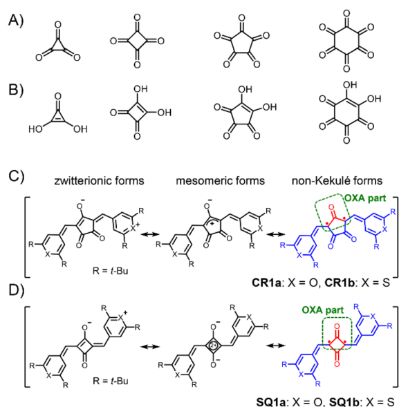
Fig. 2 Neutral oxocarbons ( \text{CO}_n ) (A). Conjugated acids of oxocarbon dianions ( \text{CO}_n^{2-} ) (B). General resonance structures including zwitterionic, mesomeric, and non-Kekulé forms for the present croconaine dyes ( CR1a–b , C) and squaraine dyes ( SQ1a–b , D). Non-Kekulé diradical parts are shown in red. Oxyallyl (OXA) parts are shown in a green round box.
