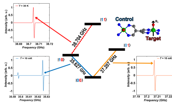
Fig. 5 Plots of the calculated frequency-swept spectra with a magnetic field of 1.3 T applied along the local z axis of the target vanadyl moiety in three different regions, corresponding to inverting the electronic spin of the control (blue line, bottom left corner), of the target without inverting the control (orange plot, bottom right corner) and of the target once the control is inverted (red plot, upper left corner). A temperature of 10 mK is employed to simulate thermal initialization in the ground state, while T = 30 K is employed to have a sizeable intensity of the transition of the target once the control is flipped (red).
