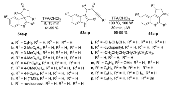
Scheme 18 Synthesis of spiro-indolenines 54a–p and quinoline analogs 55a–p .
