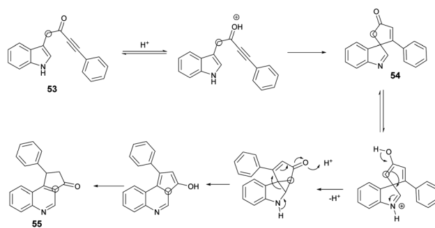
Scheme 19 Plausible mechanism for the synthesis of spiro-indolines and quinolines.
