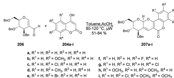
Scheme 72 Synthesis of pyrano[3,2-c]pyranone hybrids 207a-i fused with 2-C-formyl galactal.
