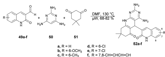
Scheme 17 Synthesis of dihydropyrido[2,3- d ]pyrimidines 52a–f .
