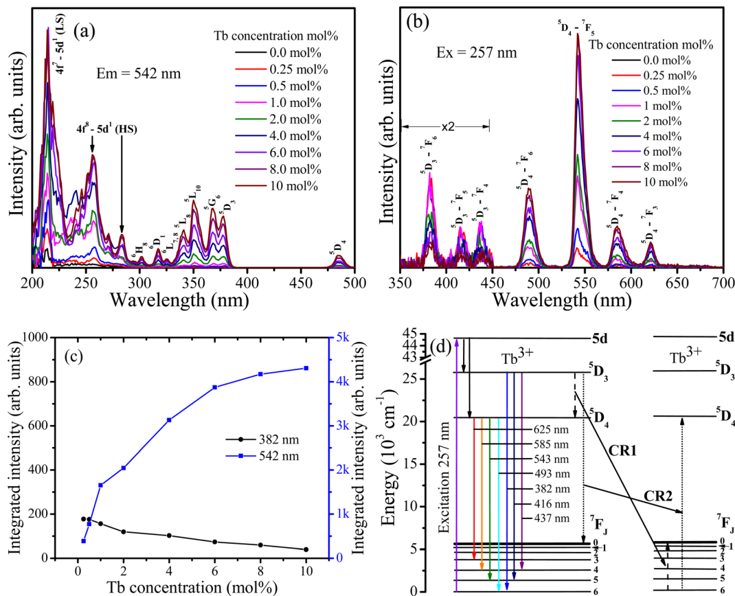
Fig. 6 PL spectra of undoped and Tb 3+ doped CaF 2 nanoparticles. (a) Excitation spectra monitored for emission at 542 nm. (b) Emission spectra excited at 257 nm. (c) Integrated intensity of the bands at 382 nm and 542 nm as a function of Tb 3+ concentration. (d) Energy diagram representation of Tb 3+ ions in CaF 2 host as well as the cross-relaxation paths.
