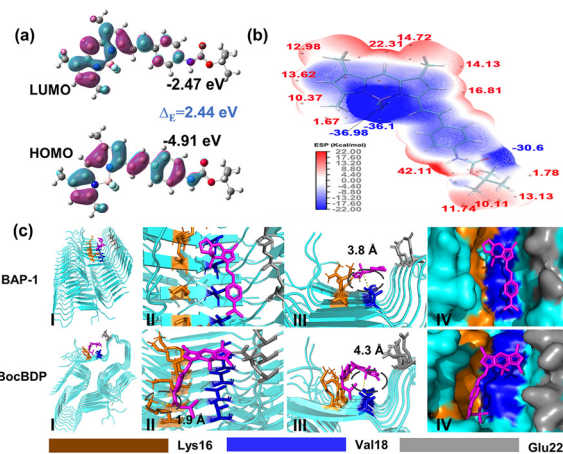
Fig. 2 Theoretical calculations and molecular docking results. (a) The highest occupied molecular orbital (HOMO) and the lowest unoccupied molecular orbital (LUMO) of BocBDP. (b) The surface electrostatic potential of BocBDP. (c) The docking results of BAP-1 and BocBDP. (I) The global view of molecular docking. (II) Licorice form of the molecule in the A \beta_{1-42} aggregate model. (III) The average distance between the probe and the amino acid residues of the pocket. (IV) Molecular surface form of the molecule in the A \beta_{1-42} aggregate model.
