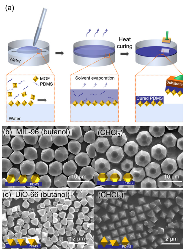
Fig. 16 (a) Scheme of preparation of oriented MOF–PDMS films. (b) SEM images of oriented MIL-96–PDMS films prepared using butanol (left) and \text{CHCl}_3 (right) as a casting solvent. Adapted with permission from ref. 101. Copyright 2021, American Chemical Society.
