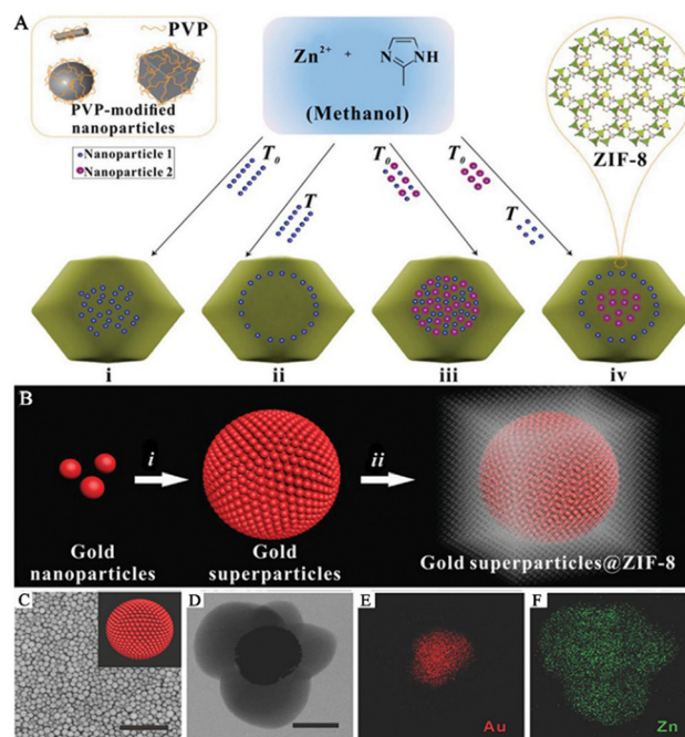
Fig. 2 Composite materials of PNPs/MOFs with core-shell structure. (A) A schematic diagram of a controlled encapsulation strategy to prepare NPs@ZIF-8. 48 Reproduced with permission from Springer Nature, copyright 2012. (B) A schematic diagram of the preparation of GSPs@ZIF-8. Scale bar: 1 \mu\text{m} . (C) SEM image of the GSPs. Inset: the schematic diagram of GSPs. (D) TEM image of the GSPs@ZIF-8. Scale bar: 100 nm. (E and F) Energy-dispersive X-ray elemental map of GSPs@ZIF-8. 14 Reproduced with permission from John Wiley and Sons, copyright 2018.
