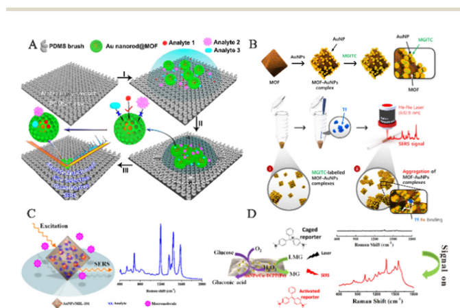
Fig. 10 Schematic diagram of MOF-based SERS sensing platforms used in human exhaled breath. (A) Schematic diagram of VOC detection via SERS spectroscopy. 14 Reproduced with permission from John Wiley and Sons, copyright 2018. (B) Schematic diagram of a SERS sensing platform for VOC detection. 41 Reproduced with permission from John Wiley and Sons, copyright 2019. (C) Schematic diagram of breath analysis using an Ag@ZIF-67-based tubular SERS sensor. 97 Reproduced with permission from American Chemical Society, copyright 2022. (D) Schematic diagram of the mask sensing device for the breath test. 40 Reproduced with permission from John Wiley and Sons, copyright 2022.
