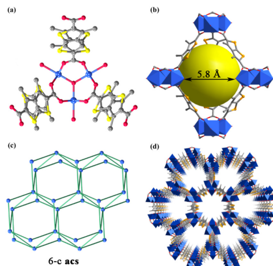
Fig. 1 The structure of Ni-MOF1. (a) The coordination environment of inorganic SBUs. (b) The cage structure. (c) The 6-connected topology network. (d) View of the 3D structures along the c axis (blue balls: Ni; red balls: O; yellow balls: S; and grey balls: C).
