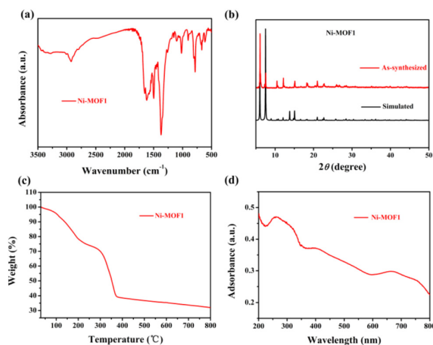
Fig. 2 Basic characterization of Ni-MOF1. (a) Infrared (IR) spectra. (b) Powder X-ray diffraction (PXRD) (black curve: single-crystal simulation and red curve: experimental synthesis). (c) TGA curves. (d) UV-vis diffuse reflectance spectra.
