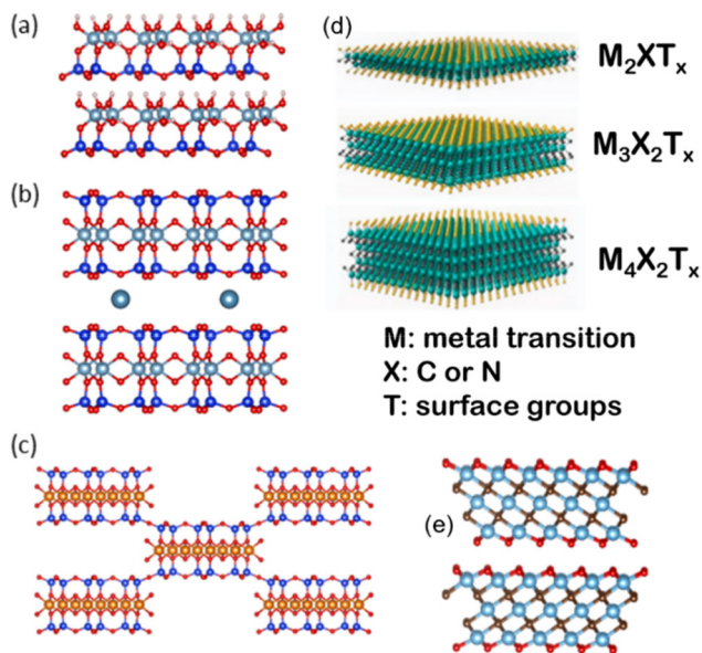
Fig. 2 Crystal structures of a selection of clay minerals (a–c) based on Al- and Mg- phyllosilicates of 1:1 type such as kaolinite (a), 2:1 type such as montmorillonite (b) and sepiolite (c), and 2D MXenes (d and e) of M_{n+1}X_nT_x , as a general formula (M = early transition metal; X = C and/or N, and T_x = OH, F surface terminations) (d). The value n = 1-4 indicates the number of transition metal layers (and carbon and/or nitrogen layers), i.e., Ti_3C_2T_x ( n = 2 ) (e). The (a), (b), (c) and (e) figures have been built using VESTA 3 software, 33 and (d) has been adapted from Wyatt et al. , 2D MXenes: Tunable Mechanical and Tribological Properties, Adv. Mater. , 2021, 33, 2007973, Wiley.
