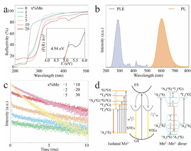
Fig. 2 (a) Diffuse reflectance spectra of CCCP: x\% Mn crystals and the plot of (F(R)h\nu)^2 versus the light energy h\nu (inset). (b) Excitation and emission spectra of the CCCP:10% \text{Mn} crystals. (c) The fluorescence decay curve of the CCCP: x\% Mn crystals ( \lambda_{\text{ex}} = 290 \text{ nm} , \lambda_{\text{em}} = 605 \text{ nm} ). (d) Schematic diagram for the photophysical processes in CCCP:Mn crystals.
