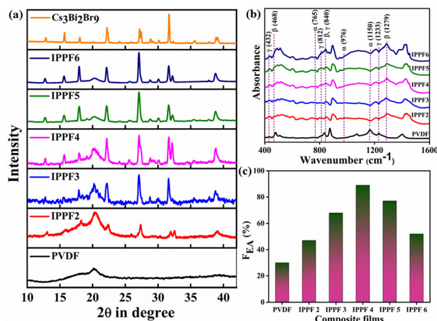
Fig. 3 (a) XRD profile, (b) FTIR spectra, and (c) the electroactive β-phase percentage of the pure PVDF and the composite samples.
